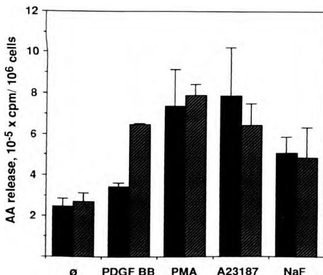
Fig. 4. Release of [\text{H}] AA in control and hPLC- \gamma_2 over-expressing cells. Control (11 \beta , filled bars) and hPLC- \gamma_2 over-expressing (13 \alpha , hatched bars) cells were grown as described in section 2. The media were then replaced by Hank's solution with 2% (w/v) BSA containing no stimulus ( \emptyset ), PDGF BB (50 ng/ml), A 23187 (10 \mu\text{M} ), PMA (1 \mu\text{M} ) or NaF (30 mM NaF/50 \mu\text{M} \text{AlCl}_3 ). After 60 min the radioactivity in the supernatants was determined. Results are means \pm S.D. of three independent experiments.
